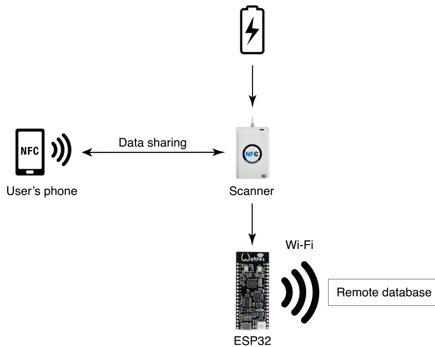
Figure 33: Final Black Box diagram
