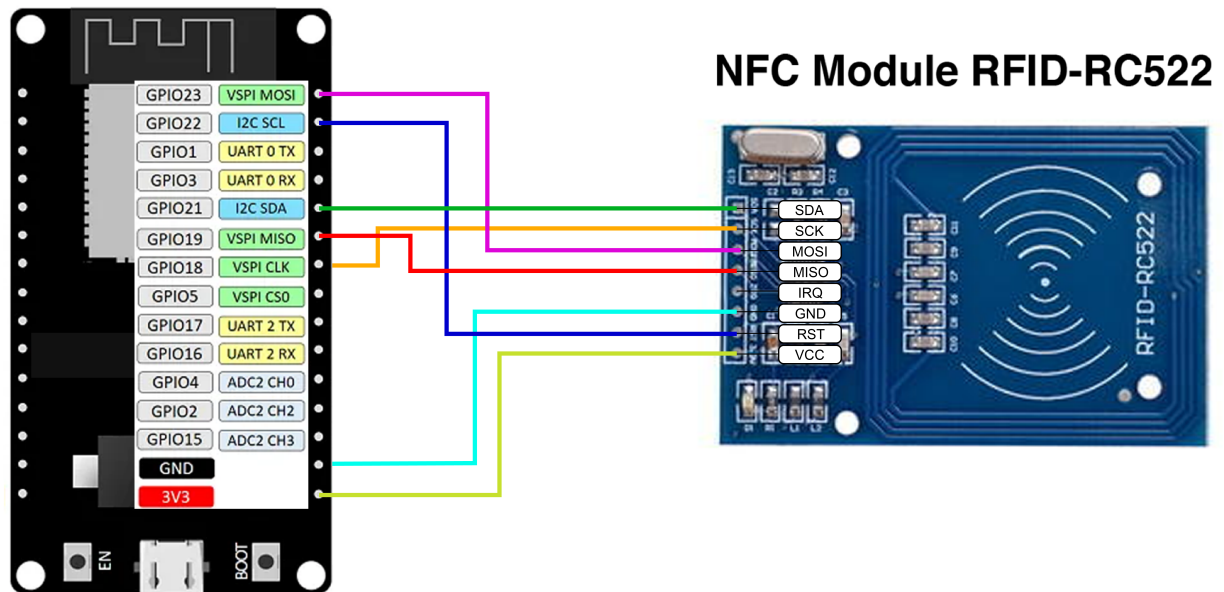
Figure 38: Pin diagram [95]
