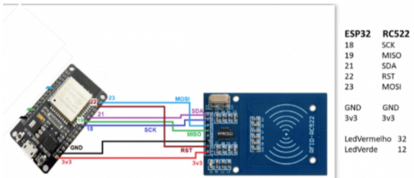
Figure 68: Connections between ESP32 and NFC module
