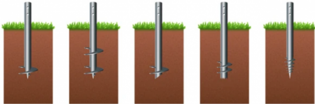
Figure 47: Ground screw anchoring [120]
