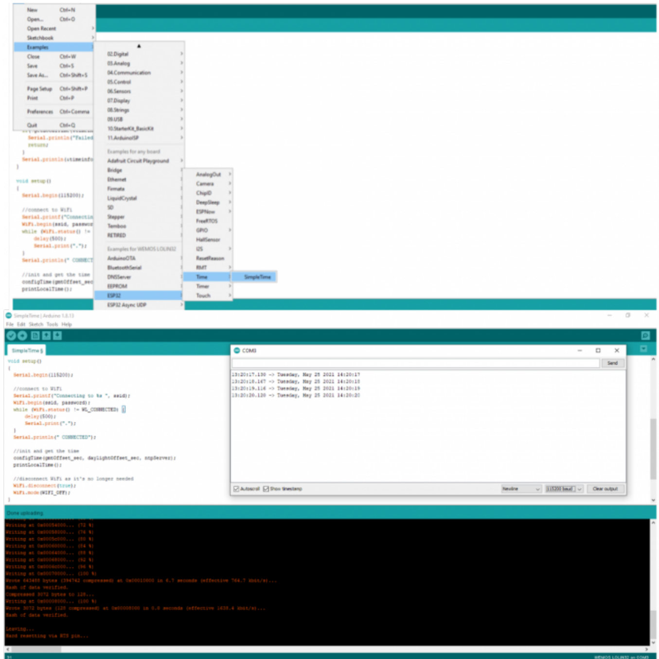
Figure 64: SimpleTime program code
