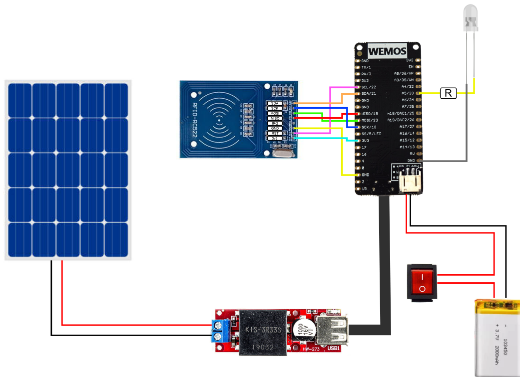
Figure 70: Circuit diagram.
