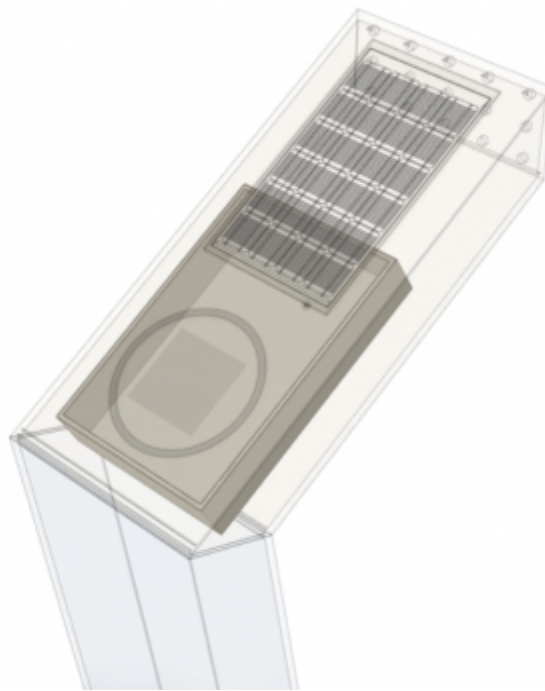
Figure 52: Components box
